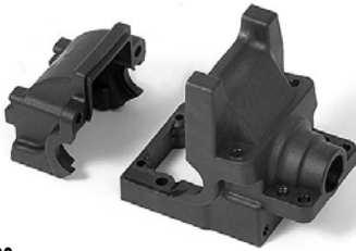
#362000 Diff Bulkhead Block Set Front - V2
